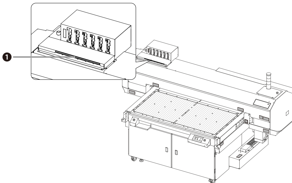
Printer Front
