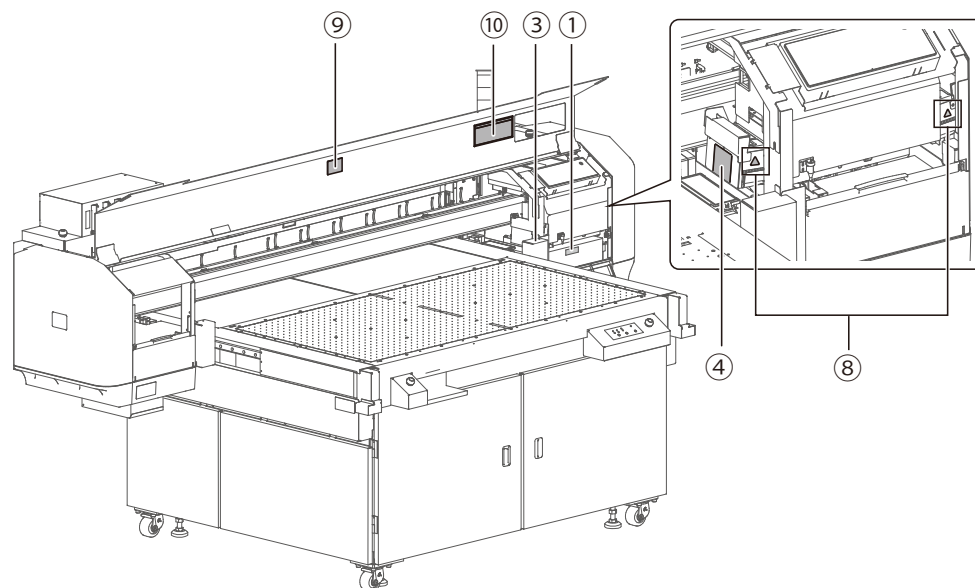
Printer Front
